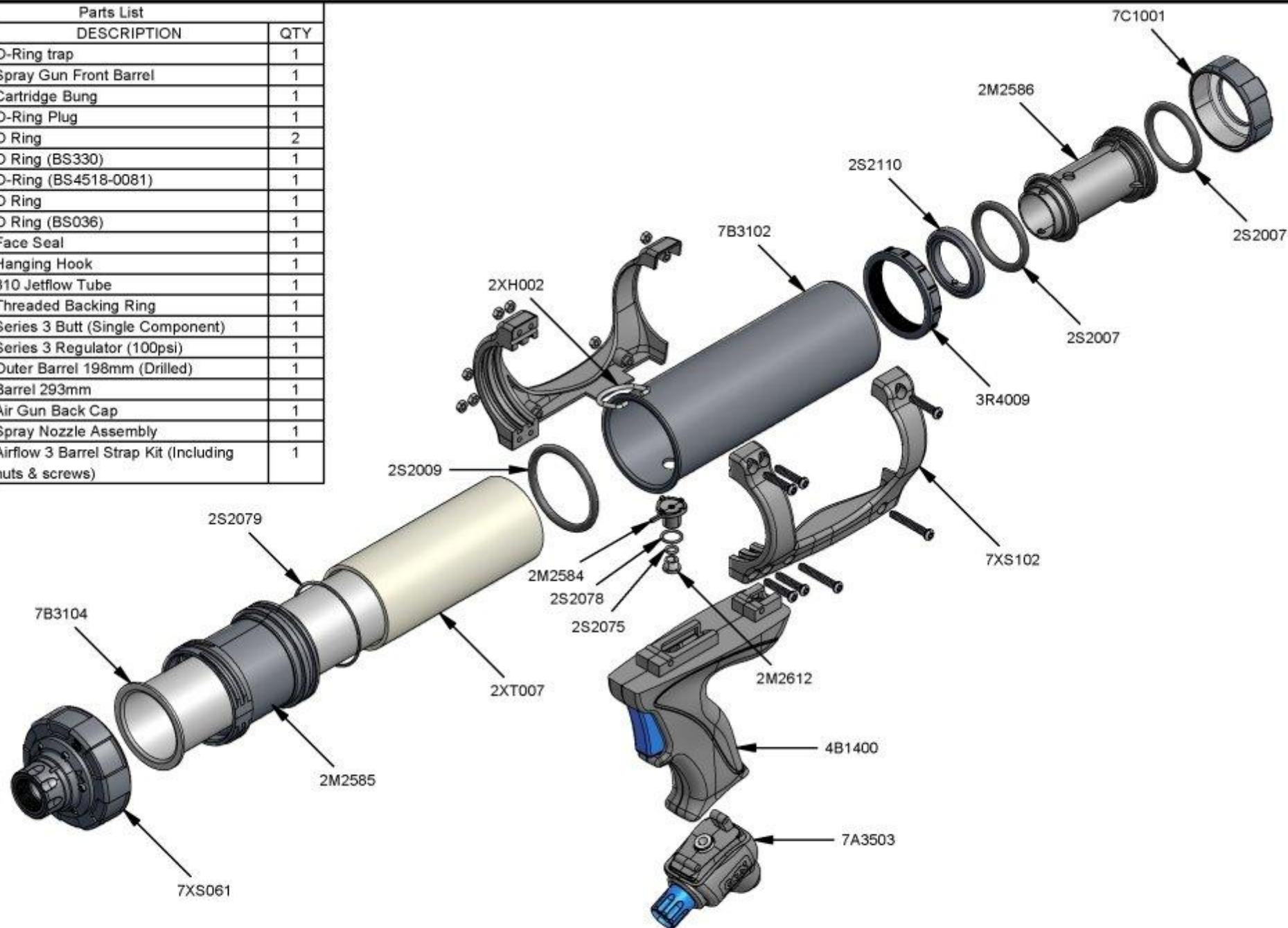
Jetflow 3 310 Cartridge
